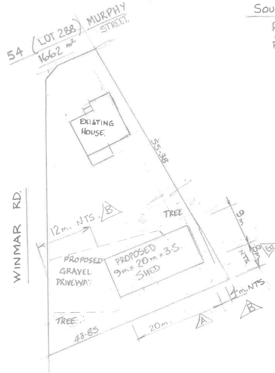
BLOCK PLAN. REV. REV.
